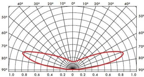
170° Lens
